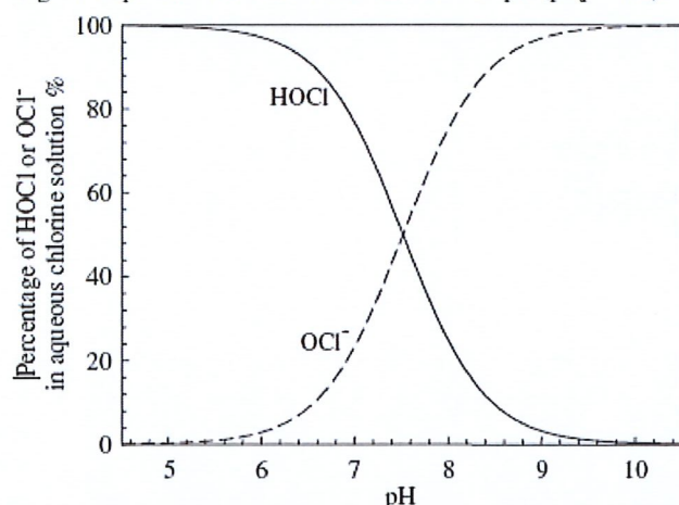
Fig. 1. Dependence of the ratio \text{HOCl}/\text{OCl}^- on pH ( \text{pK}_a = 7.5 ).
